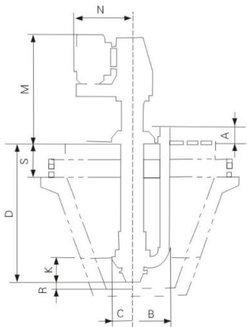
Belt Drive
